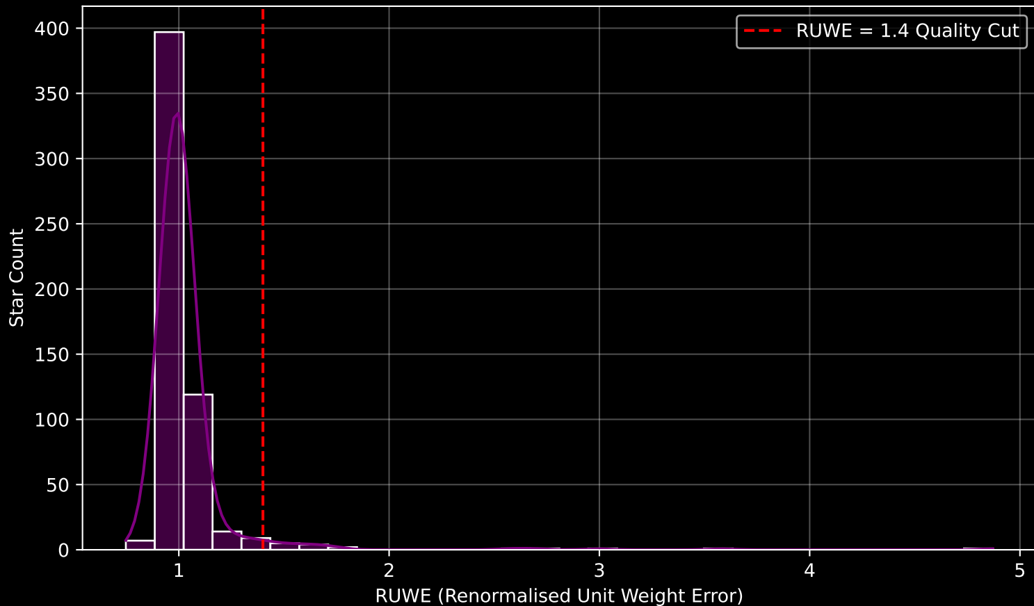
GAPOGEE DR17 Field [060+00] RUWE Distribution (n= 562)
