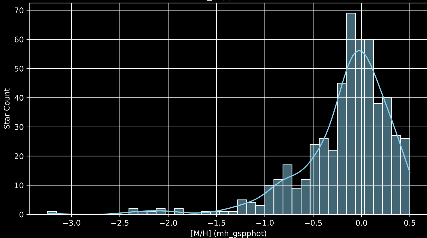
APOGEE DR17 Field: [060+00 [M/H] (mh_gspphot) (n= 522)
