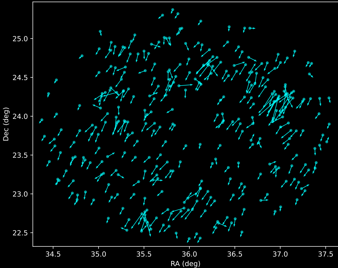
APOGEE DR17 Noise Stream Proper Motion Vectors (n=323)
