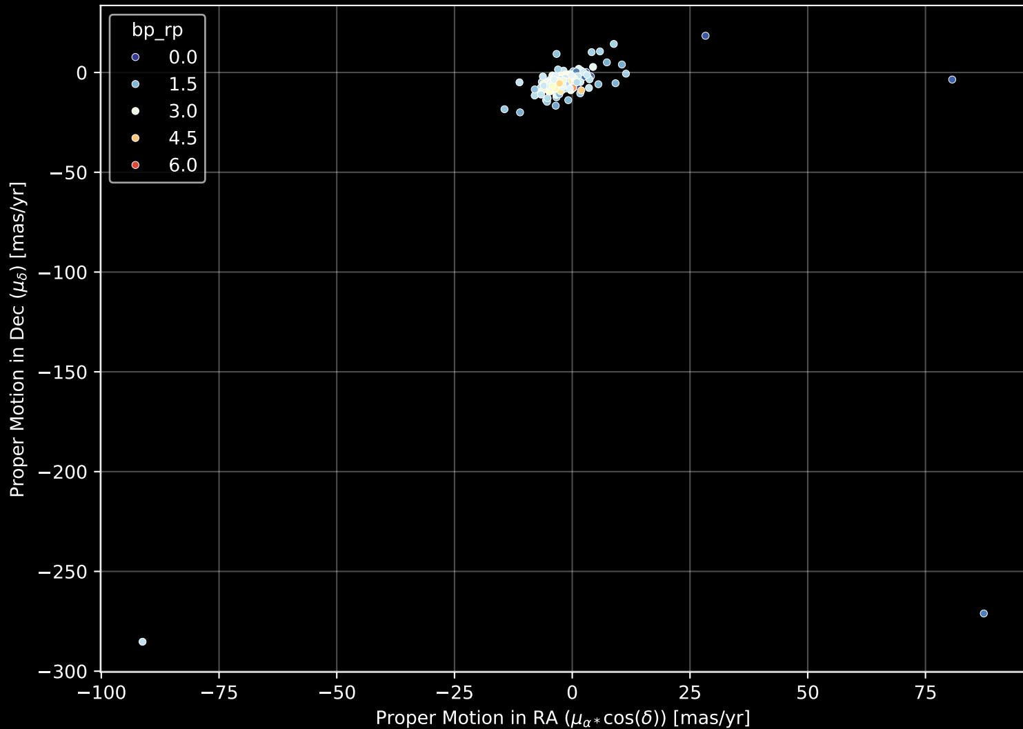
APOGEE DR17 Field: [060+00] Proper Motion Diagram (n= 563)
