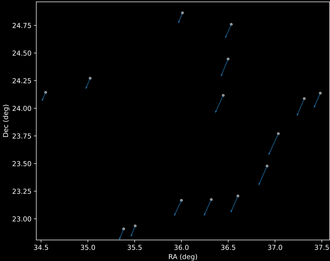
APOGEE DR17 Cluster 20 Proper Motion Vectors (n=15)
