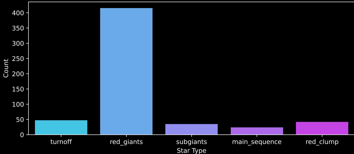
APOGEE DR17 Field: [060+00] Count plot of Star Type
