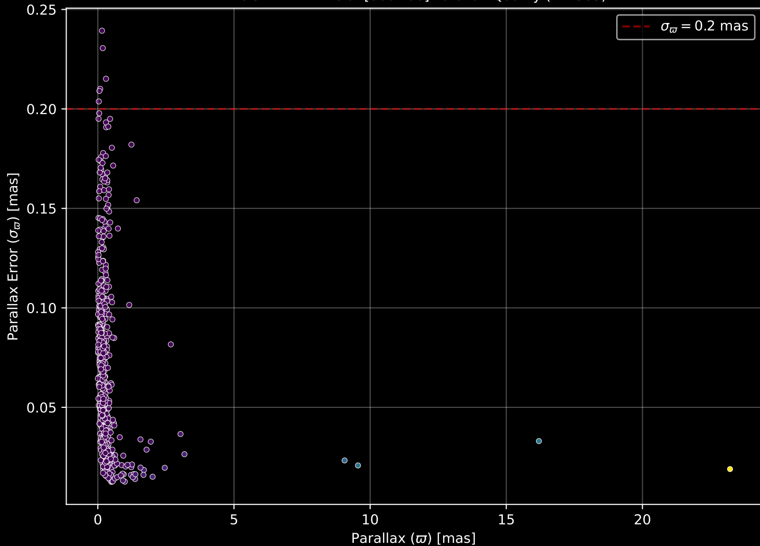
APOGEE DR17 Field: [060+00] Parallax Quality (n= 563)
